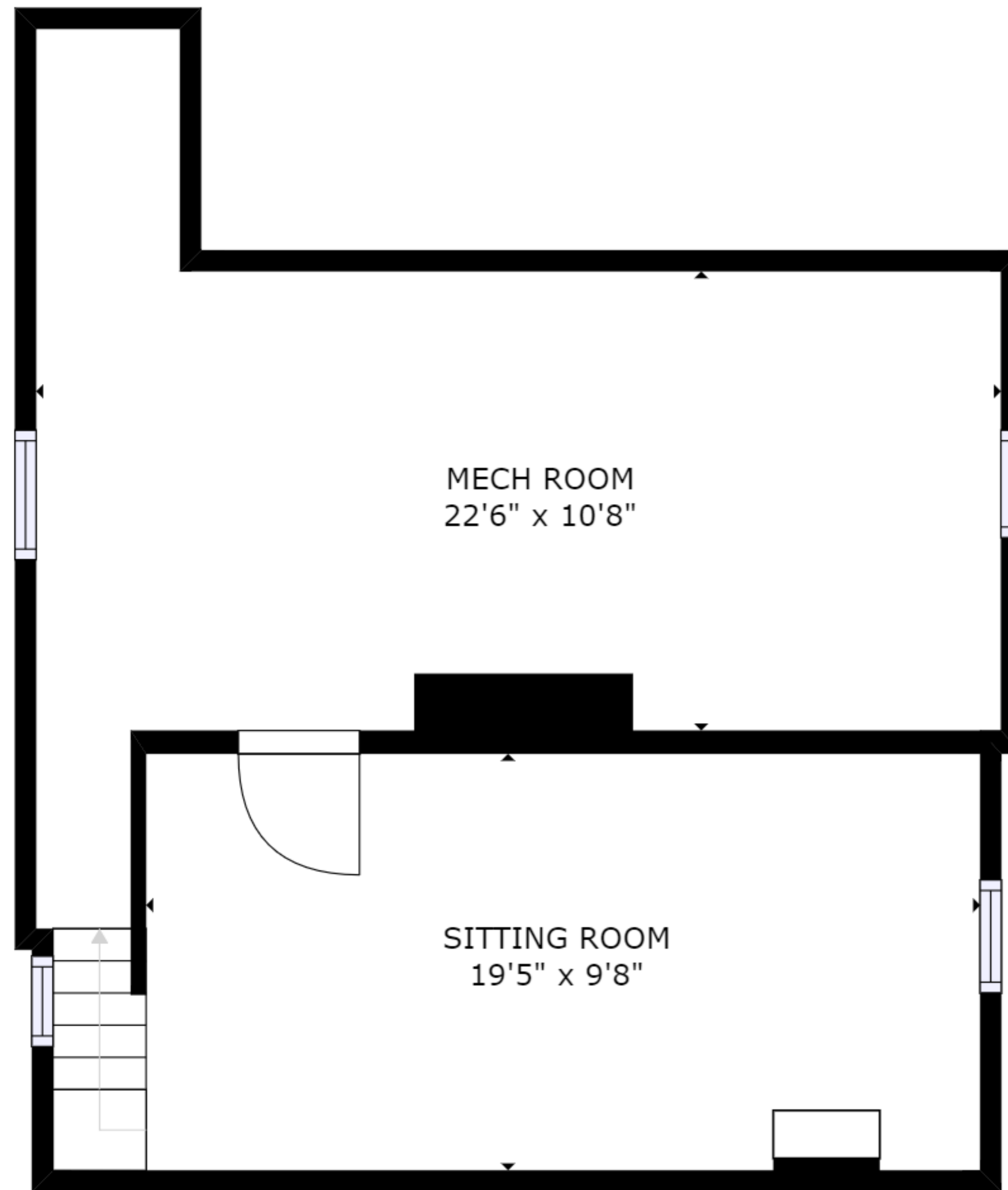
FLOOR 1
