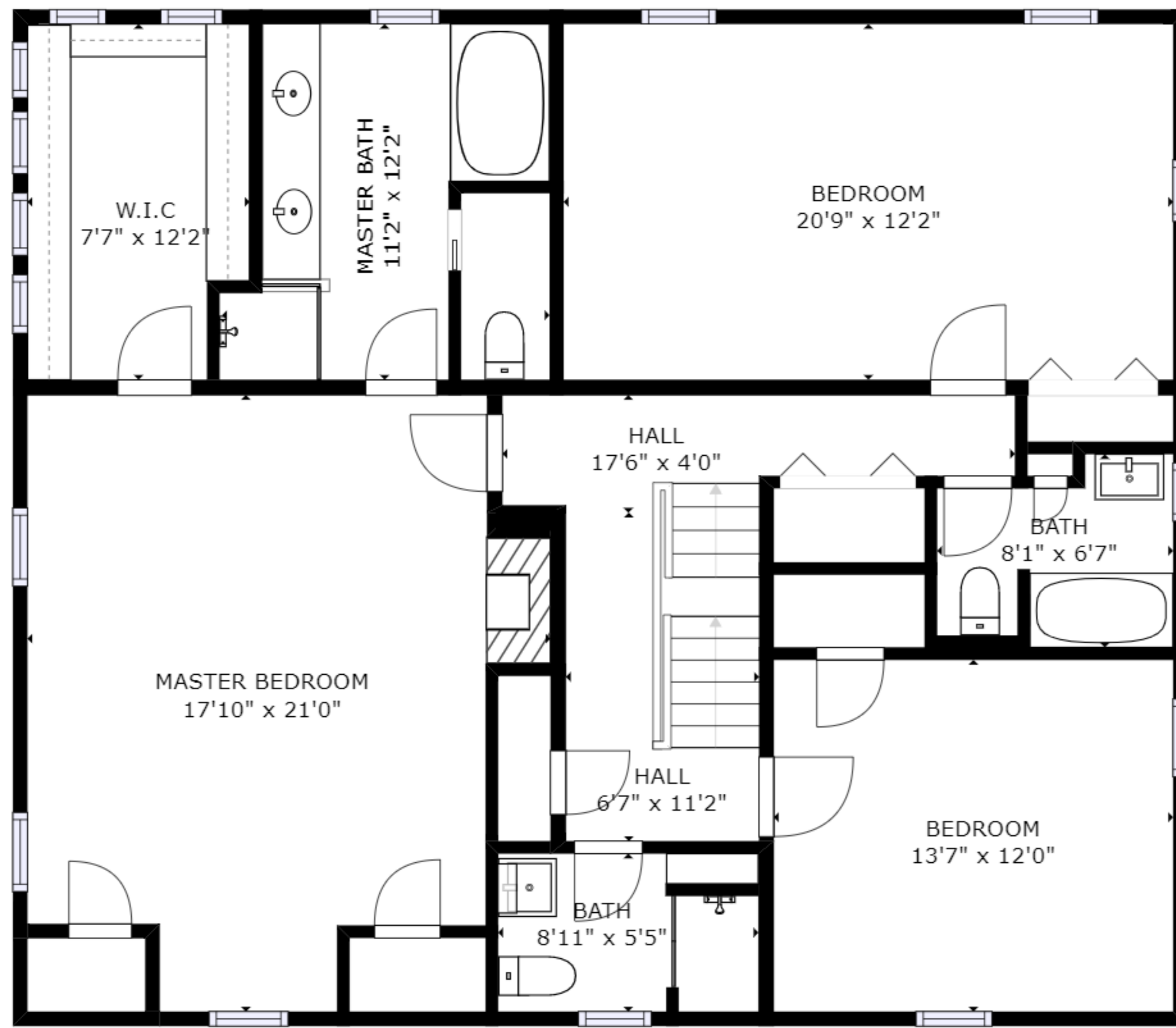
FLOOR 3
