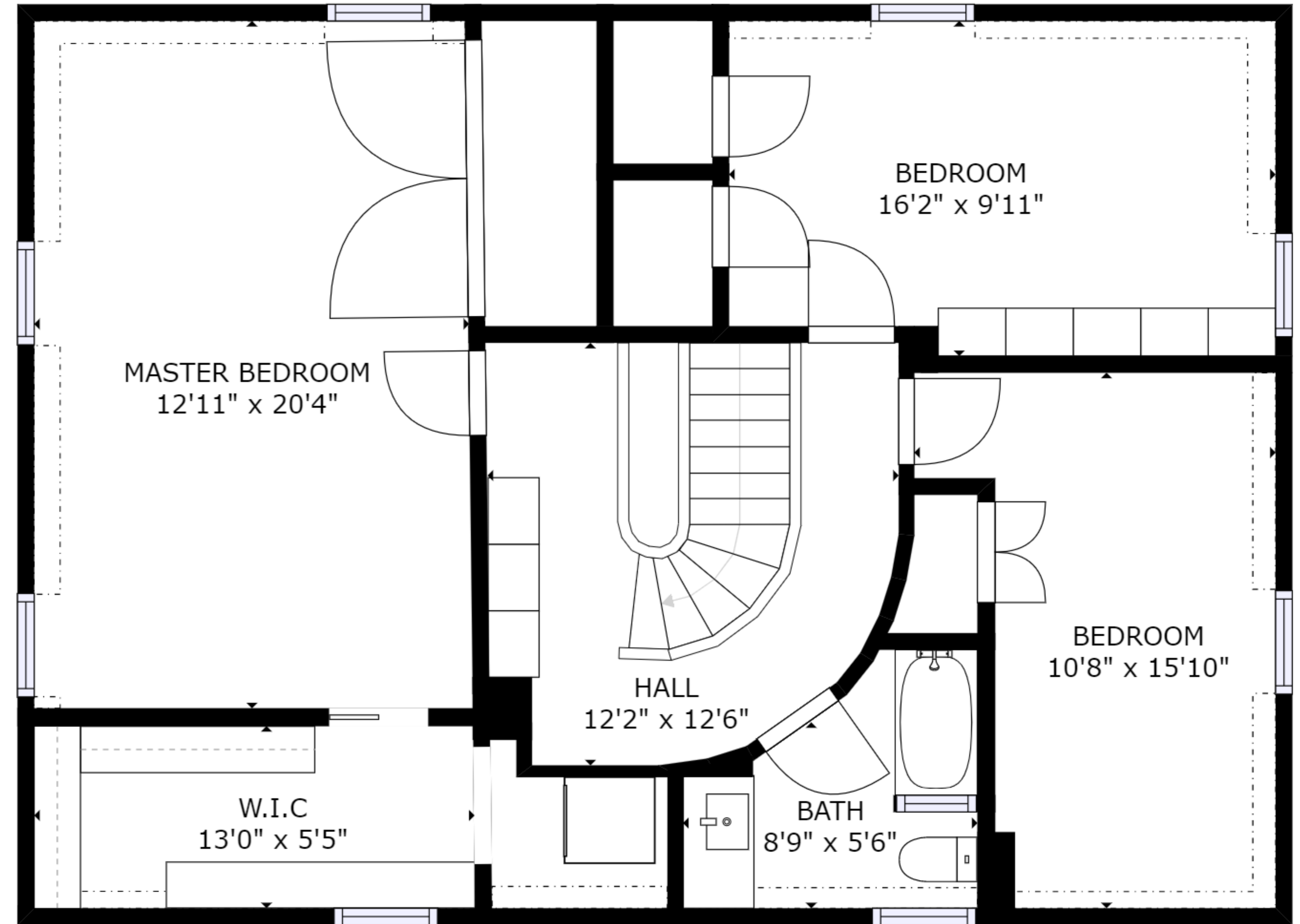
FLOOR 2
