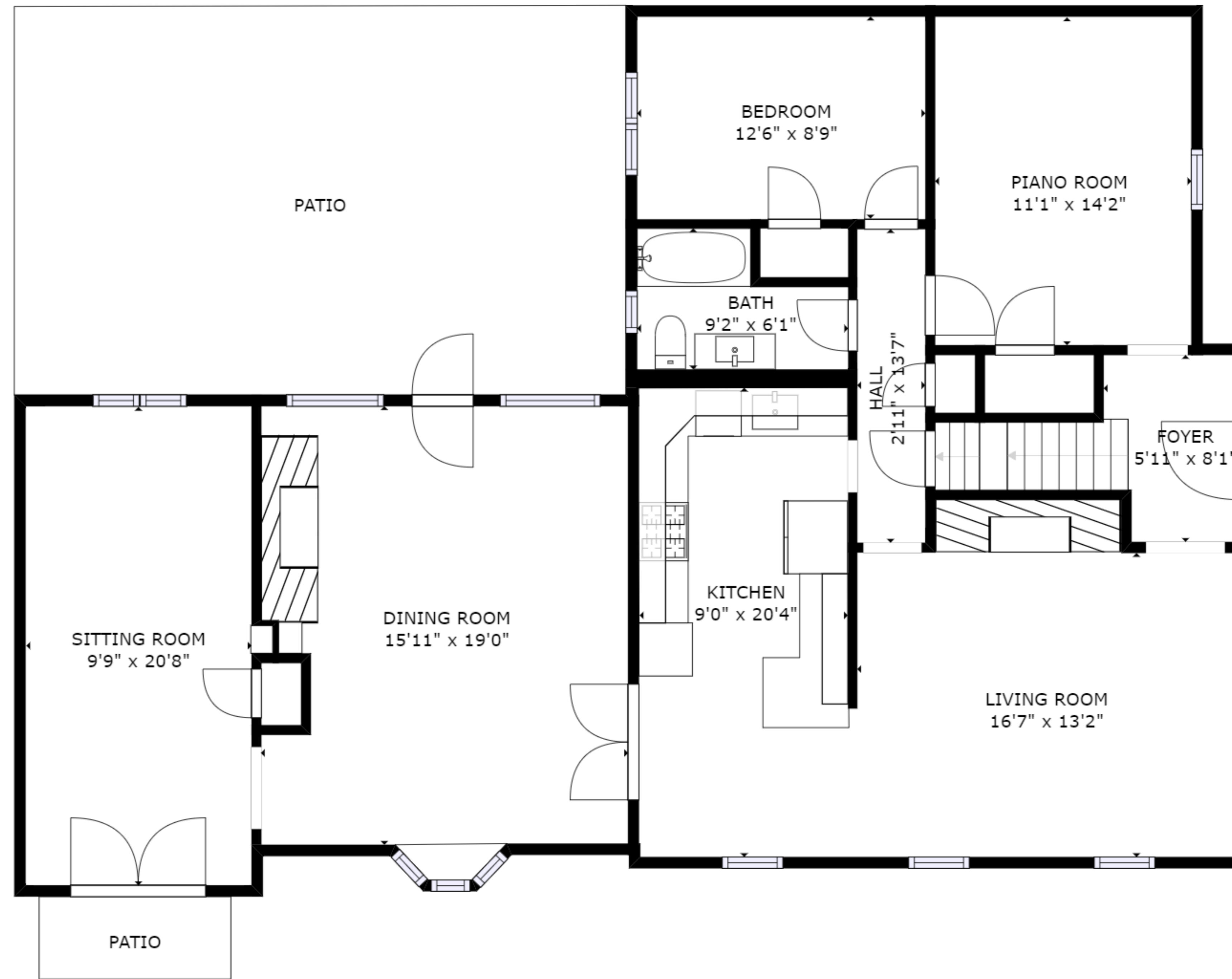
FLOOR 2
