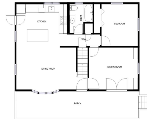
FLOOR 2
