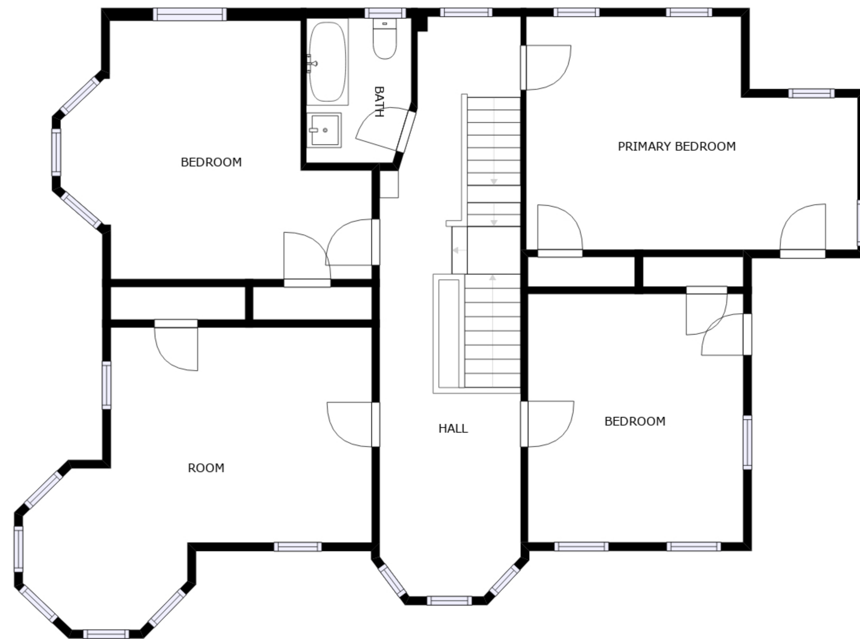
FLOOR 3
