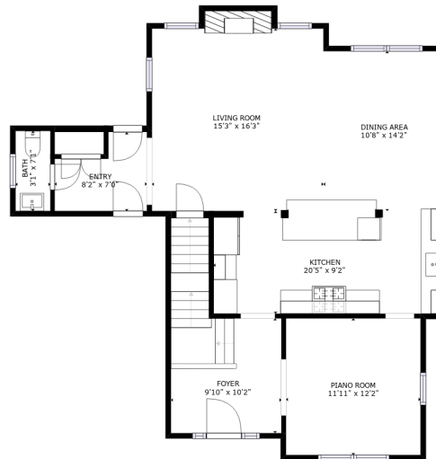
FLOOR 2
