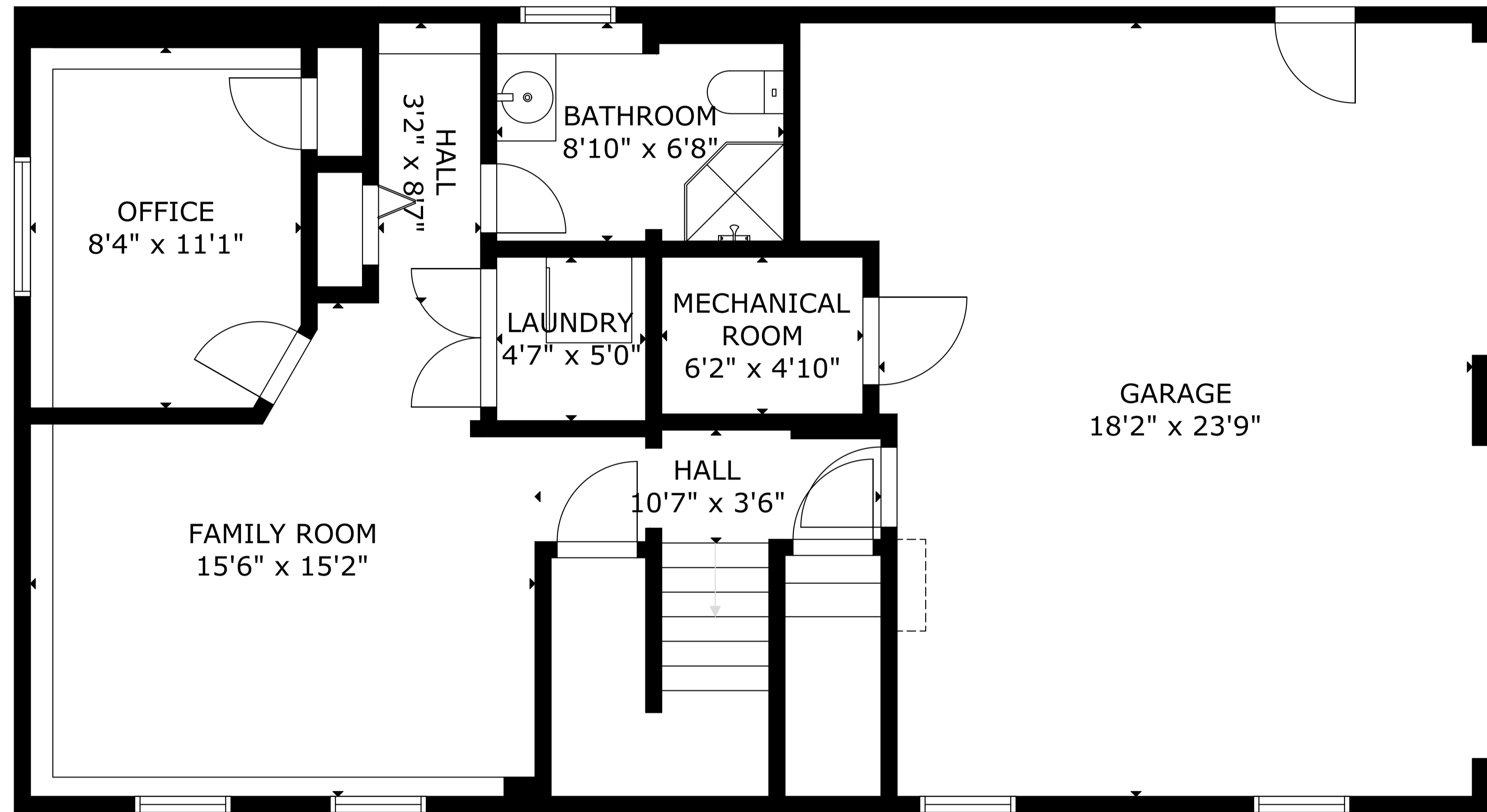
BASEMENT
