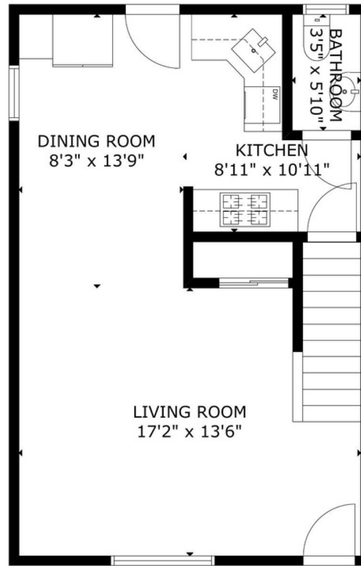
FIRST FLOOR
