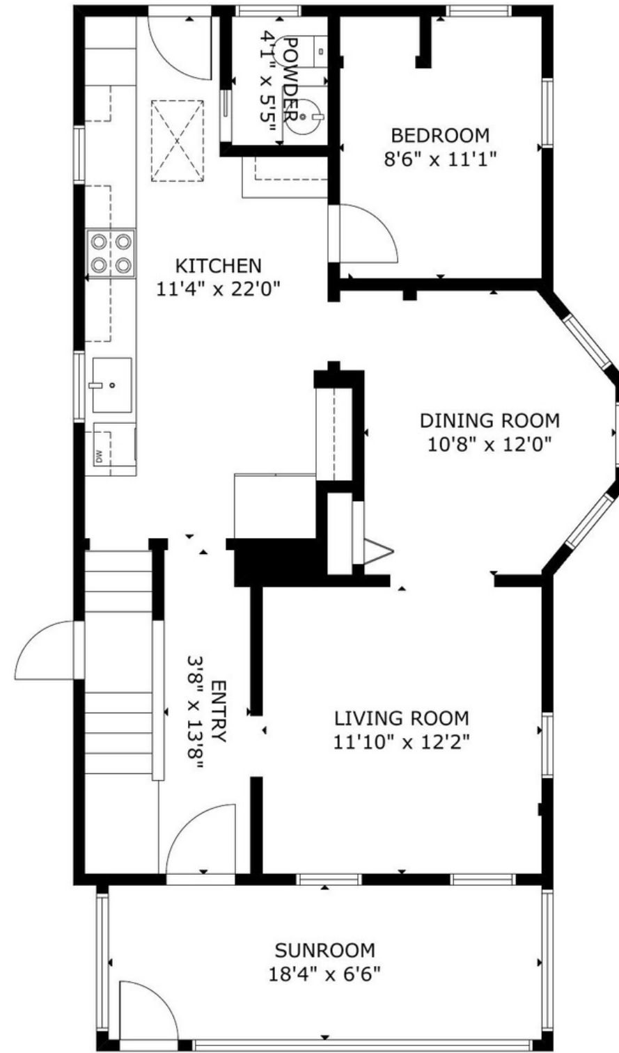
FIRST FLOOR
