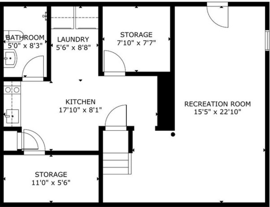
BASEMENT
