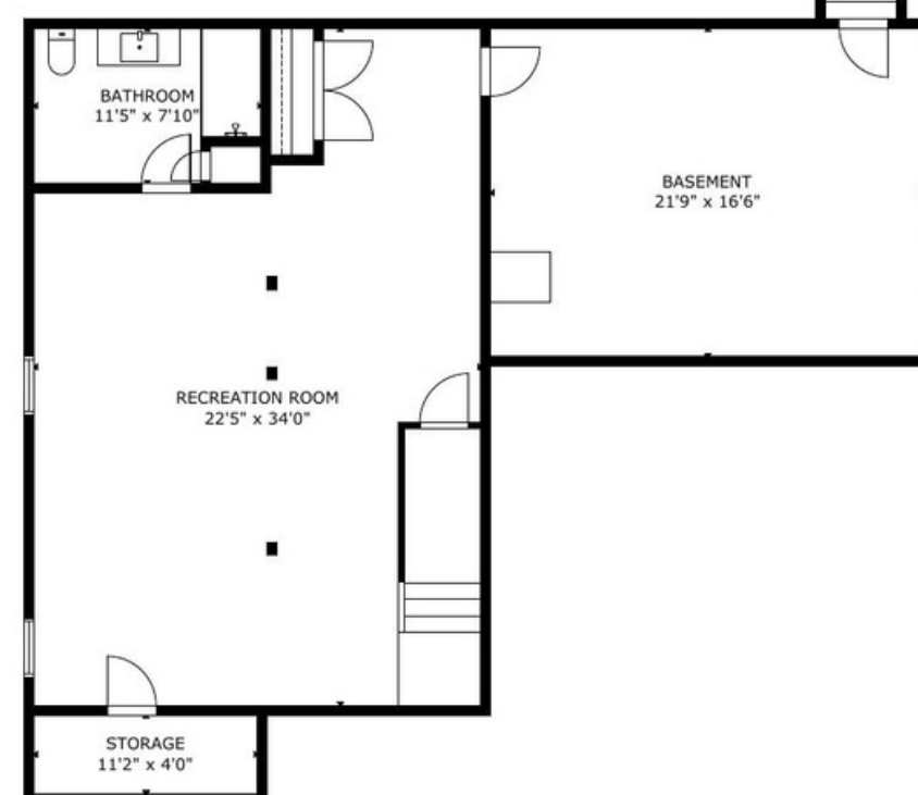
BASEMENT
