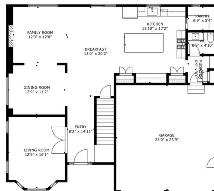
FIRST FLOOR
